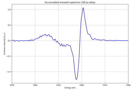
(b) Difference spectrum at a delay of 100 ps.
