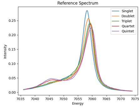
Figure 6: The reference spectra plotted with provided data for different spin states.
